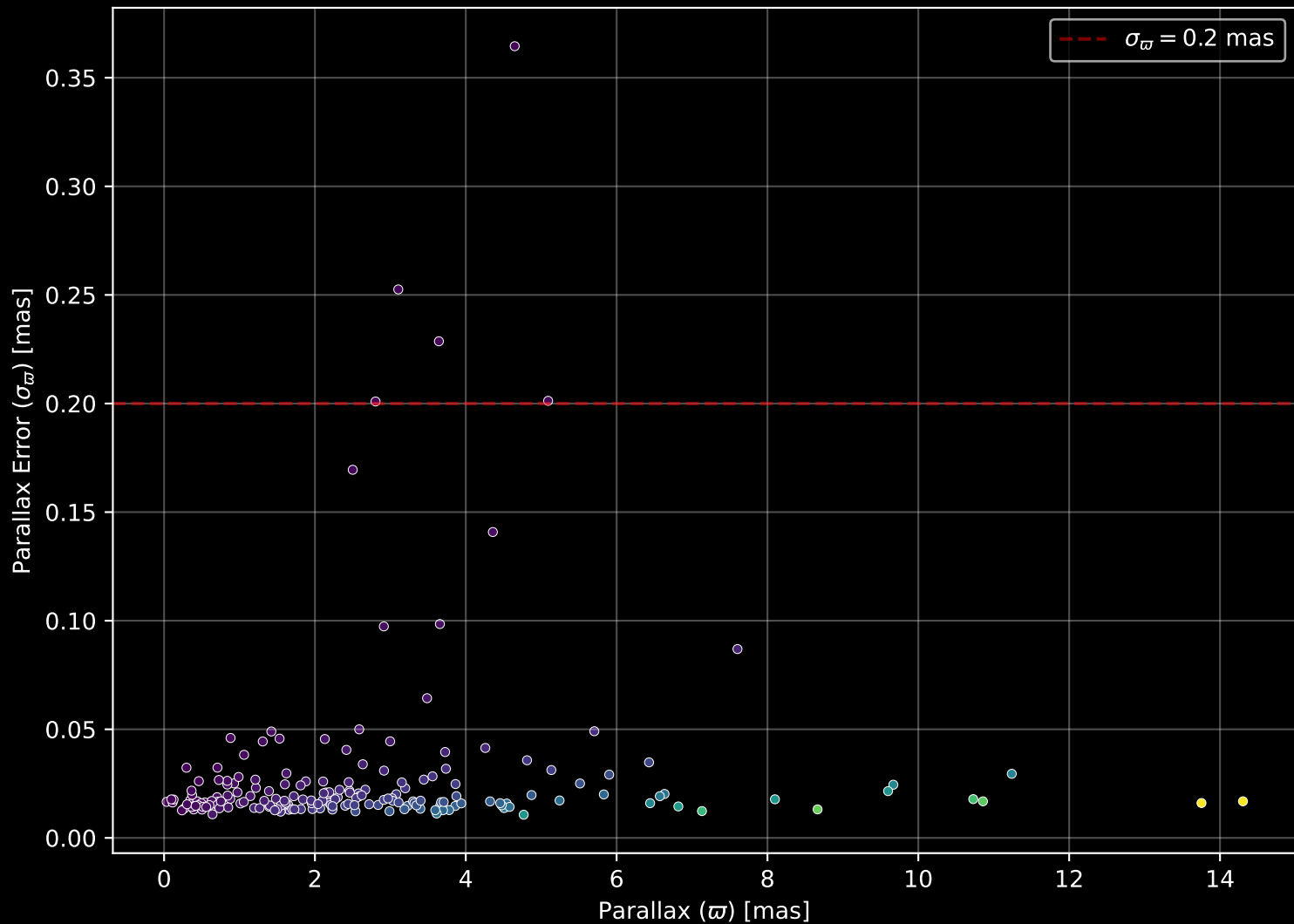
APOGEE DR17 Field: [189+27_MGA] Parallax Quality (n= 196)
