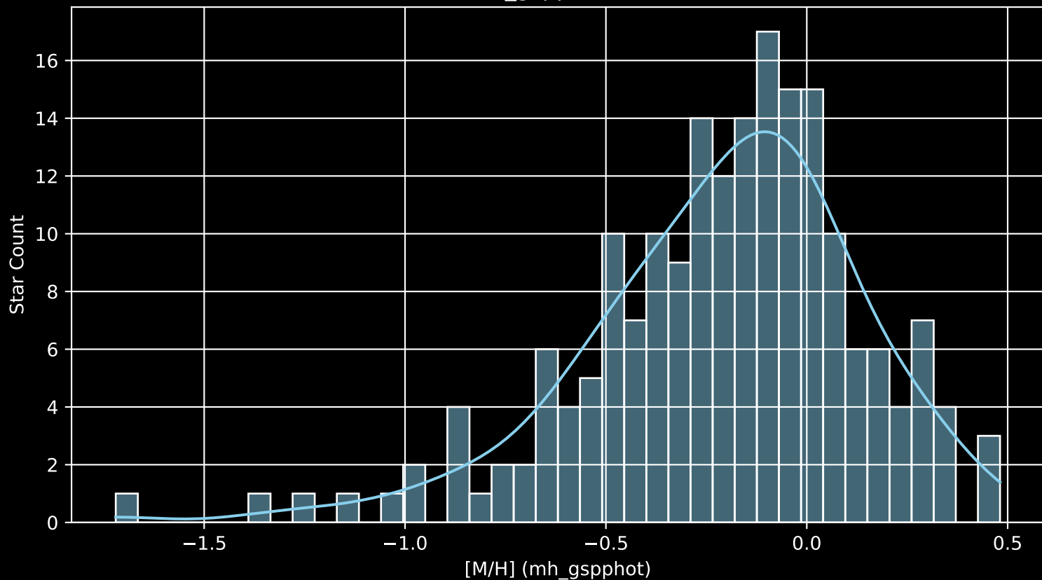
APOGEE DR17 Field: [189+27_MGA [M/H] (mh_gspphot) (n= 194)
