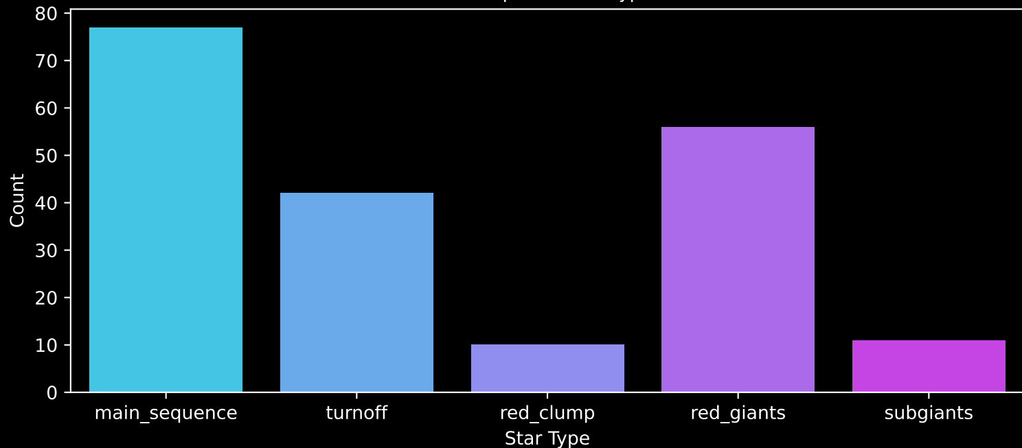
APOGEE DR17 Field: [189+27_MGA] Count plot of Star Type
