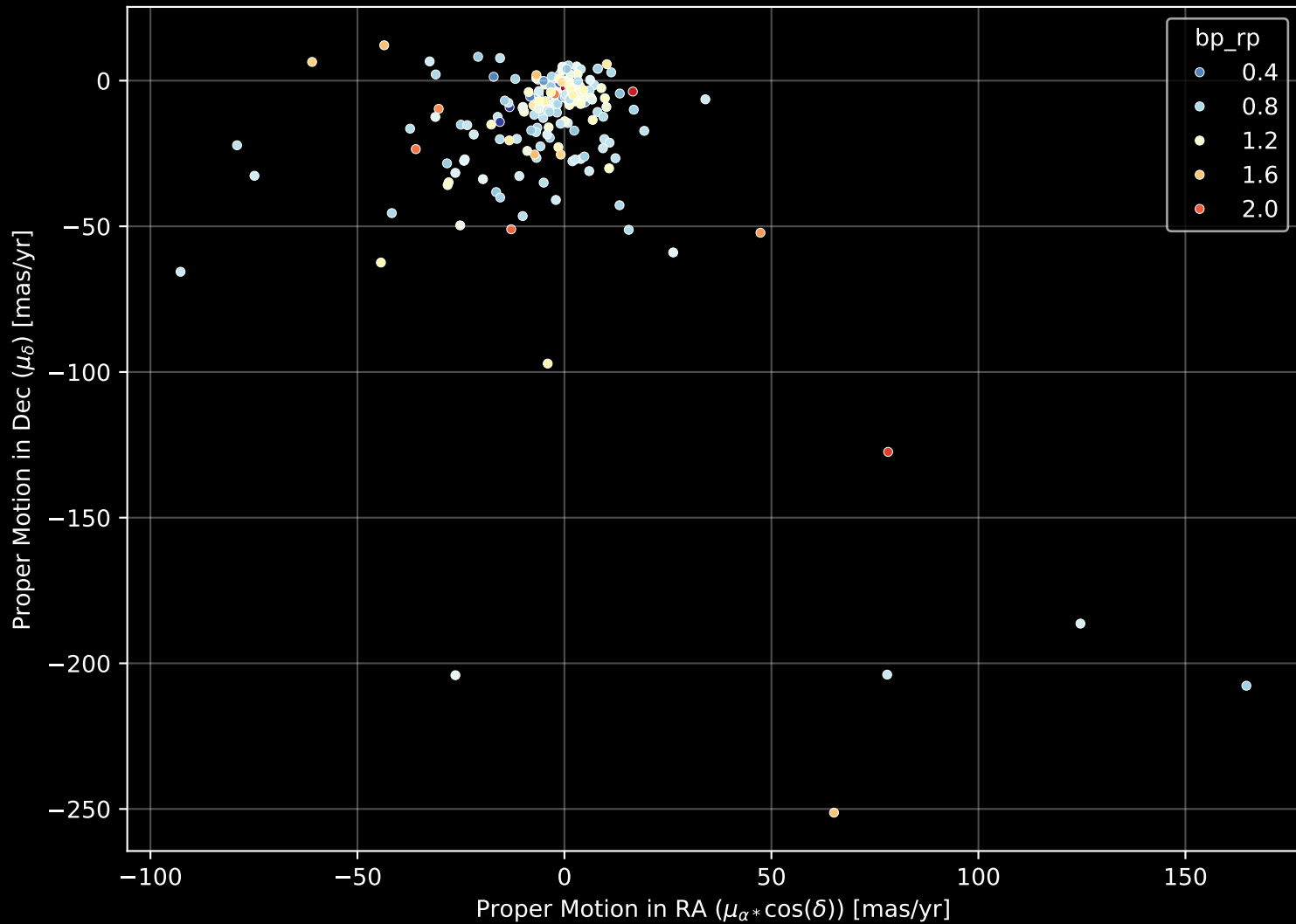
APOGEE DR17 Field: [189+27_MGA] Proper Motion Diagram (n= 196)
