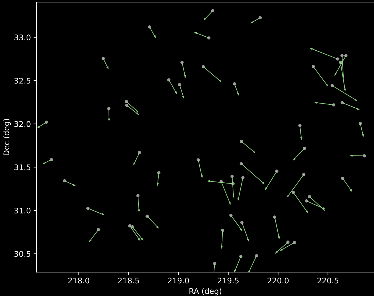
APOGEE DR17 Cluster 5 Proper Motion Vectors (n=58)
