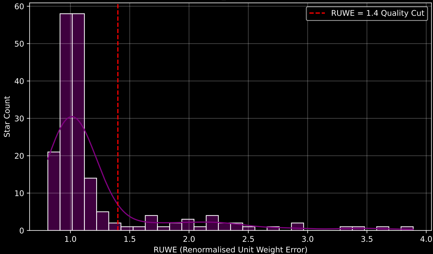
GAPOGEE DR17 Field [189+27_MGA] RUWE Distribution (n= 187)
