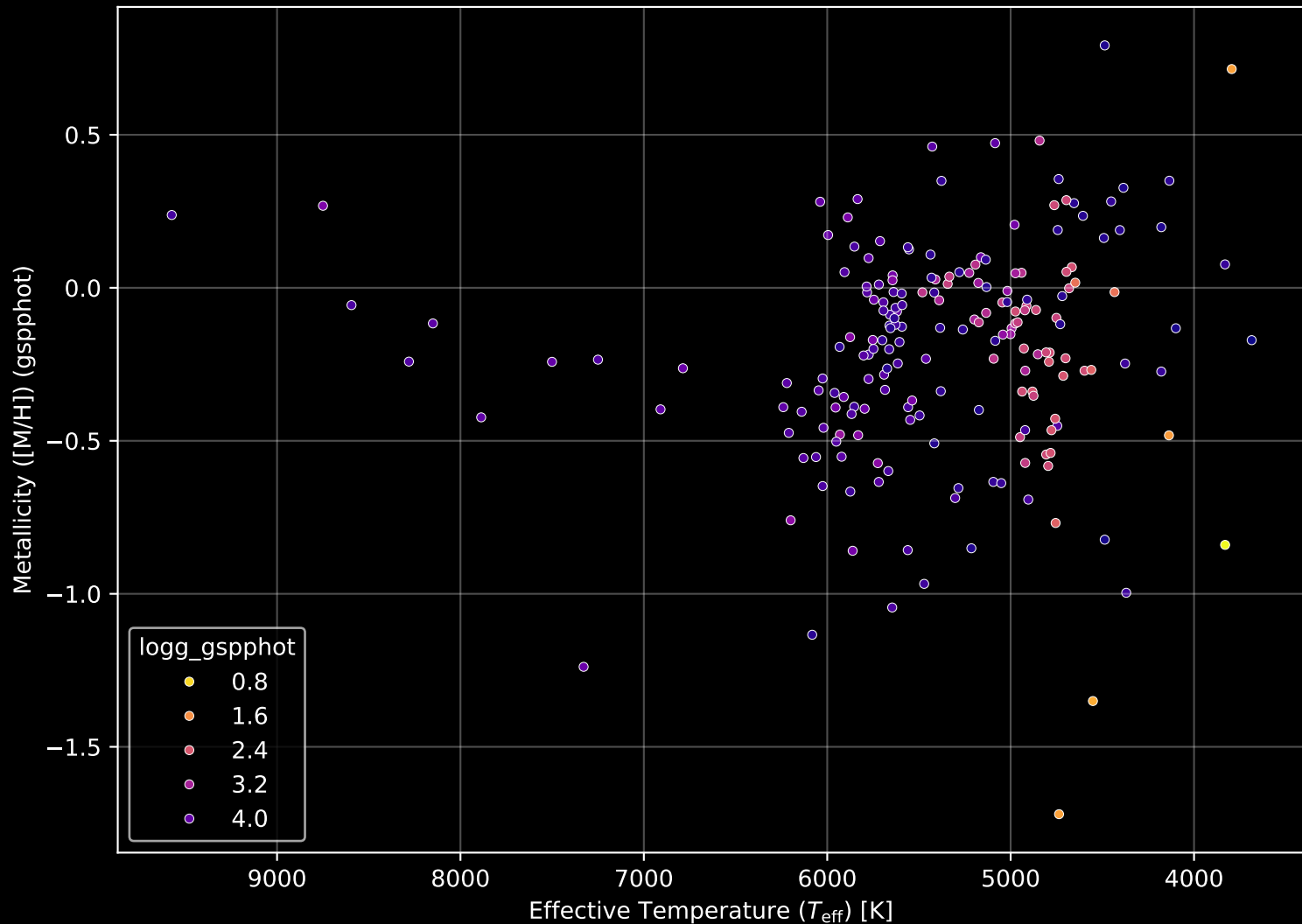
APOGEE DR17 Field: [189+27_MGA] Stellar Population Parameters (n= 196)
